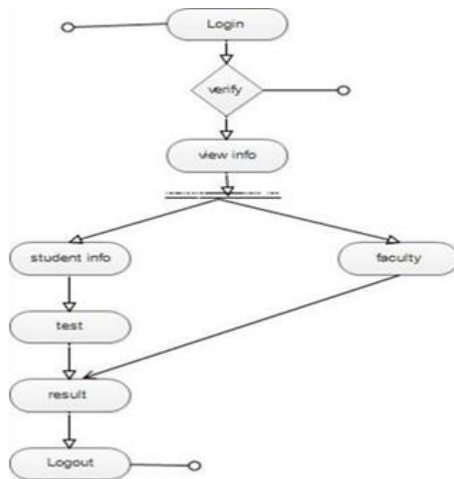
Fig 5.1 Activity Diagram
